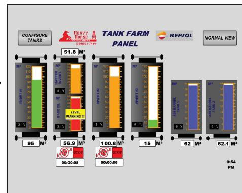
Iphone Tank Level Read Out for Horizontal Tanks
